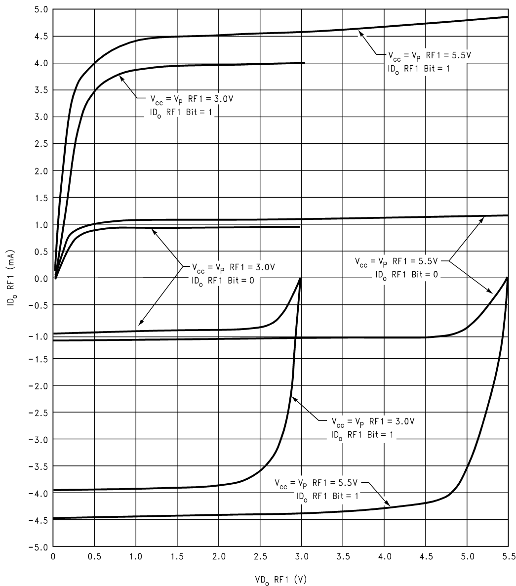
Figure 19. LMX2335U and LMX2336U RF1 Charge Pump Sweeps -40^{\circ}C \leq T_A \leq +85^{\circ}C
