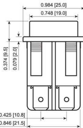
6.3mm Tab (Small Hole)
