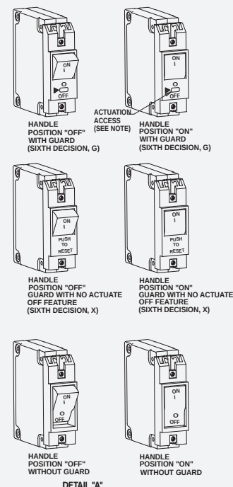
DETAIL "A"
