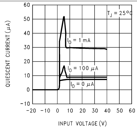
Figure 4. Quiescent Current
