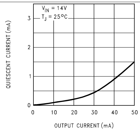
Figure 6. Quiescent Current
