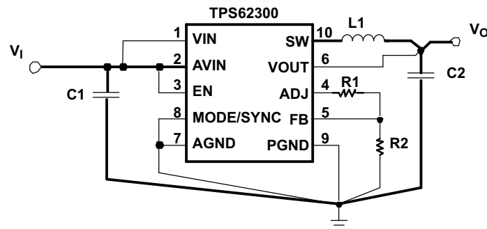
Figure 34. Layout Diagram
