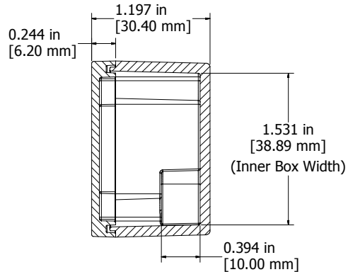
SECTION C-C End View of Assembly
