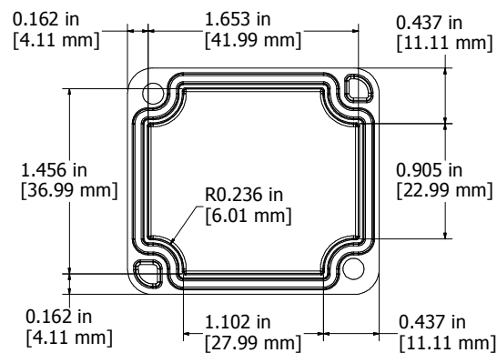
View Looking Inside Lid
