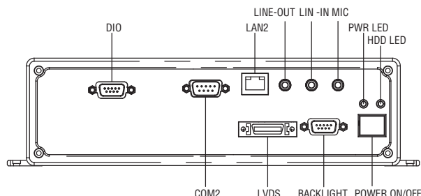
Front Panel External I/O Mechanical Layout/Drawing
