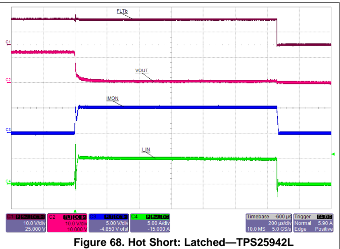
Figure 68. Hot Short: Latched—TPS25942L
