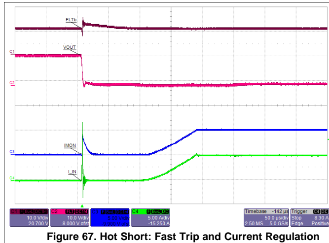
Figure 67. Hot Short: Fast Trip and Current Regulation
