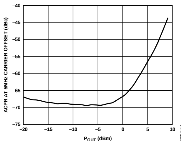
Figure 18. ACPR vs. P_{OUT} , Single W-CDMA Carrier (Test Model 1, 64) at 2140 MHz
