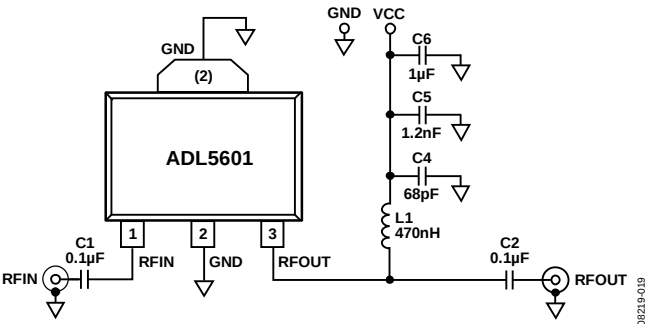
Figure 20. Evaluation Board Schematic
