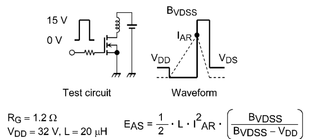
Fig. 8.16 Test Circuit/Waveform
