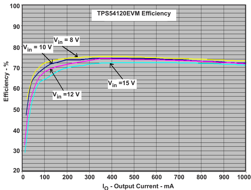
Figure 4-7. TPS54120 Efficiency
