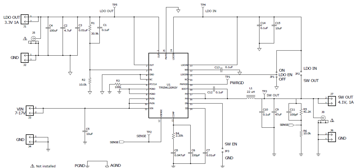
Figure 6-1. Schematic
