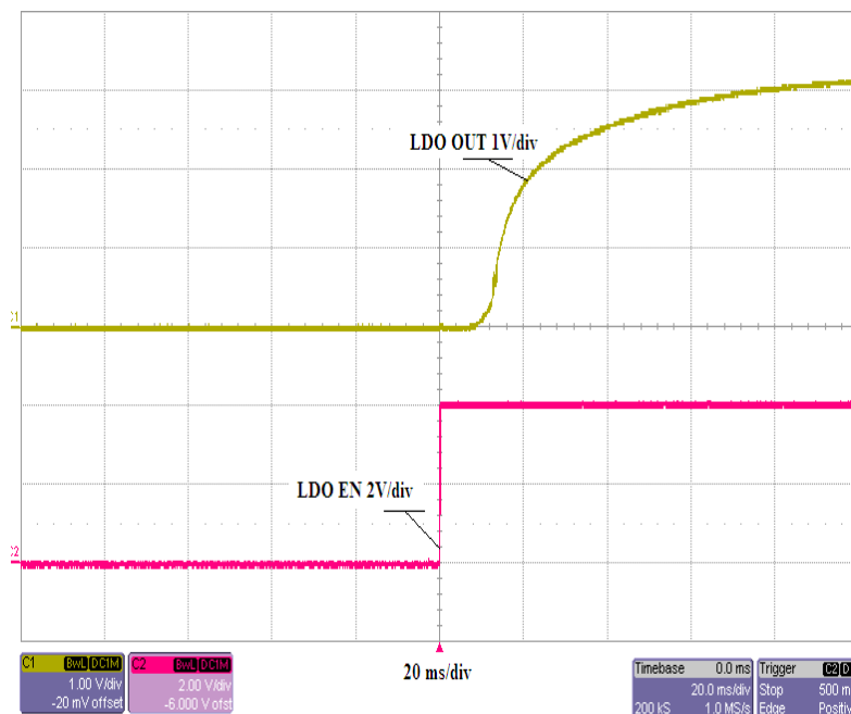
Figure 4-4. LDO Output Voltage Turn-On, LDO Enable
