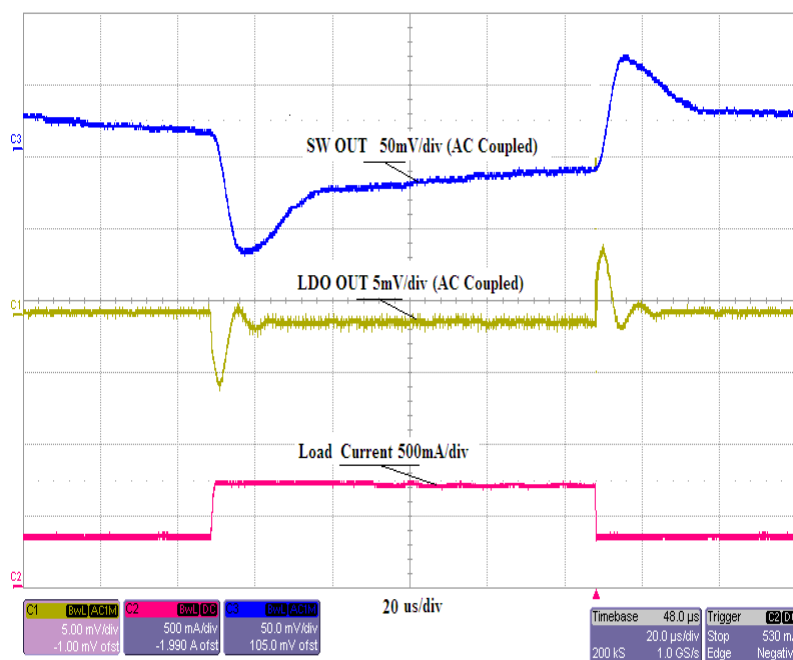
Figure 4-6. TPS54120 Transient Response
