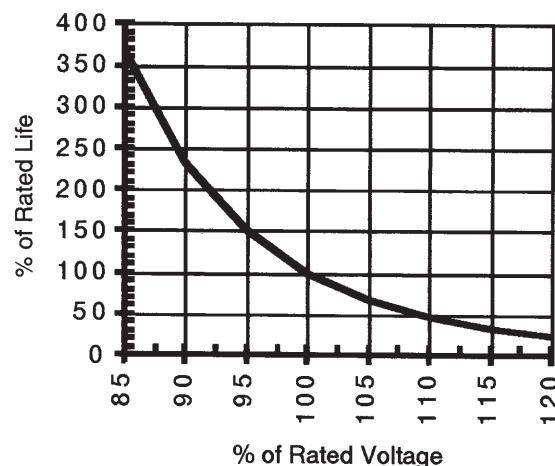
Life vs. Voltage
