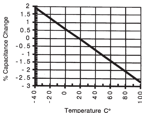
Capacitance Change vs. Temperature
