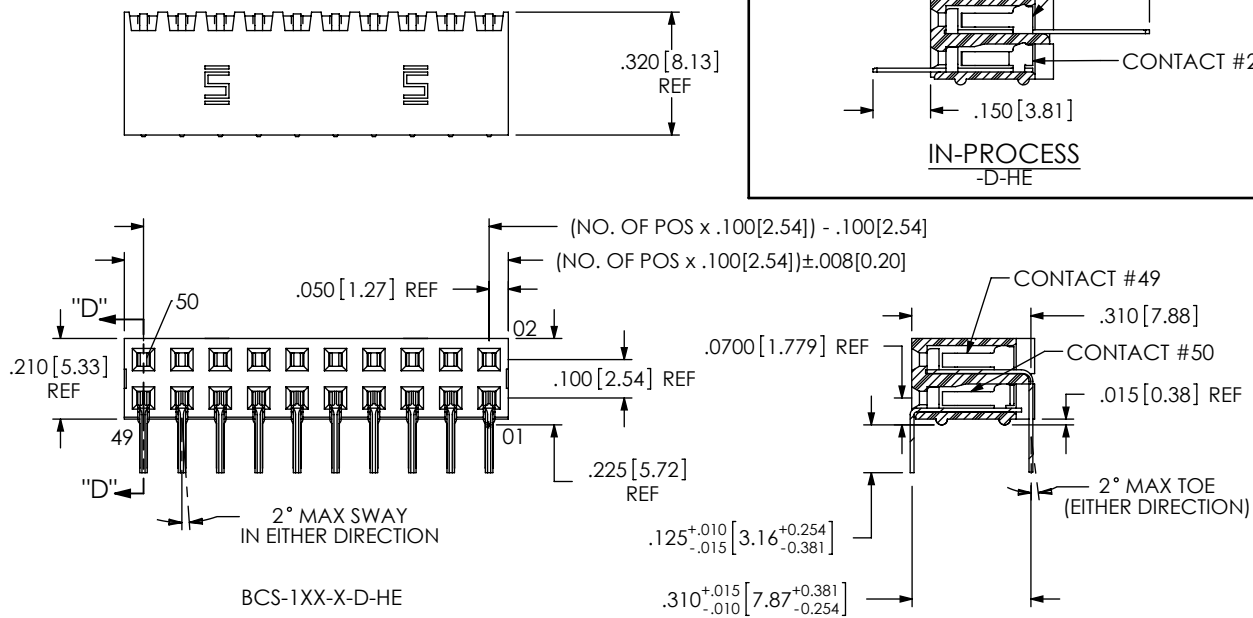
SECTION "D"-"D"
