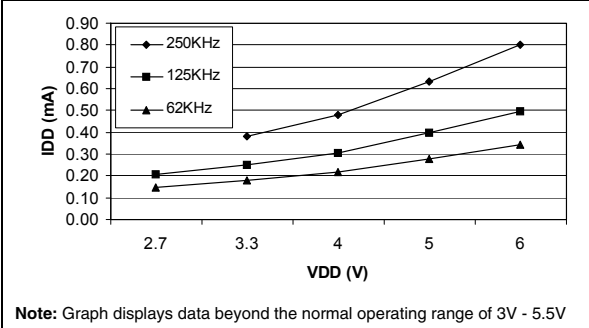
Figure 74. Typical I_{DD} in WAIT vs. f_{CPU}
