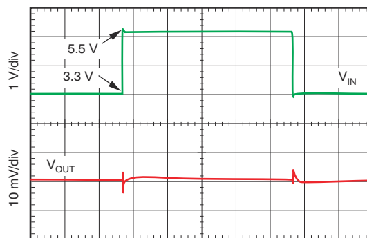
200 \mu\text{s/div} V_{OUT} = 1.8\text{ V} , I_{OUT} = 10\text{ mA}
