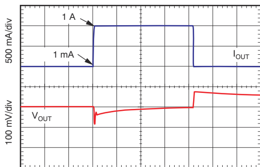
50 \mu\text{s/div} C_{OUT} = 1\text{ }\mu\text{F}
