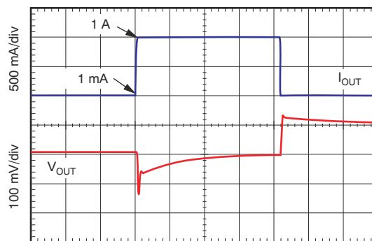
50 \mu\text{s/div} C_{OUT} = 10\text{ }\mu\text{F}
