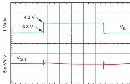
200 \mu\text{s/div} V_{OUT} = 1.8\text{ V} , I_{OUT} = 500\text{ mA}
