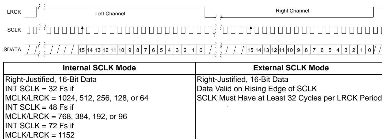
Figure 10. CS4361 Data Format (Right-Justified 16)
