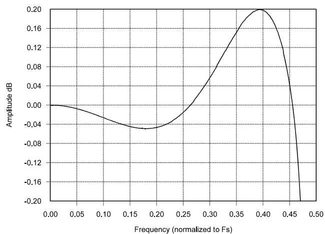
Figure 21. Double-Speed Passband Ripple
