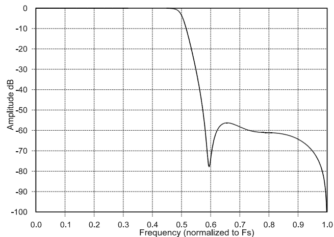
Figure 18. Double-Speed Stopband Rejection
