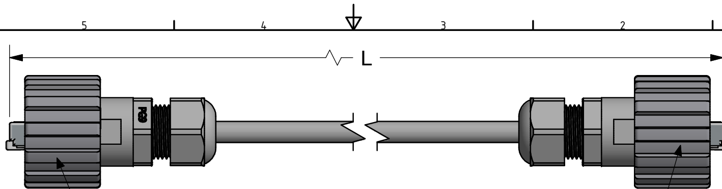
Cat. 5e RJ45 Plug (Industrial IP67, Plastic, Metallized Plastic or Die Cast version with Bayonet Locking Type)
