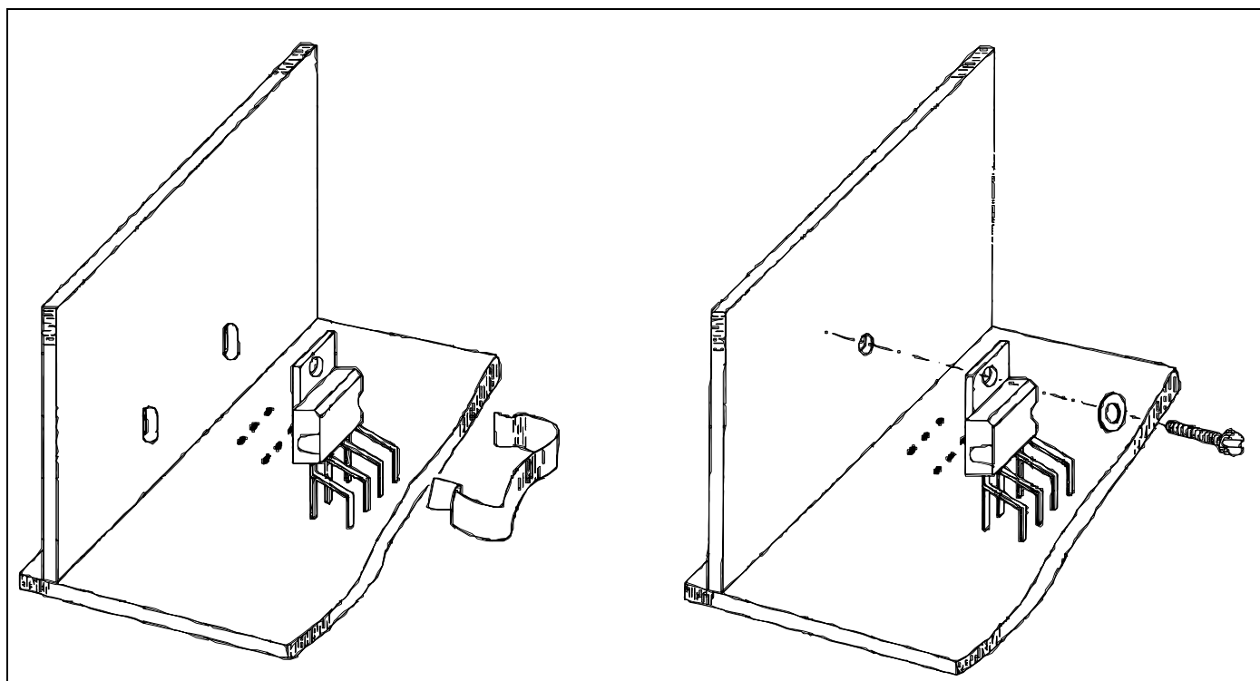
Figure 10: Mounting Examples
