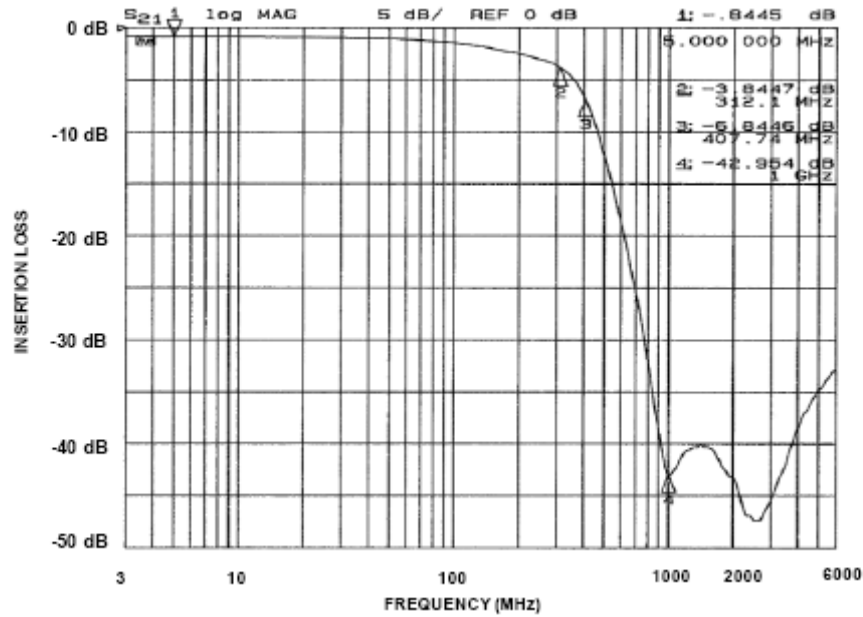
Figure 3. Insertion Loss VS. Frequency (CM1453-06: Filter 3)
