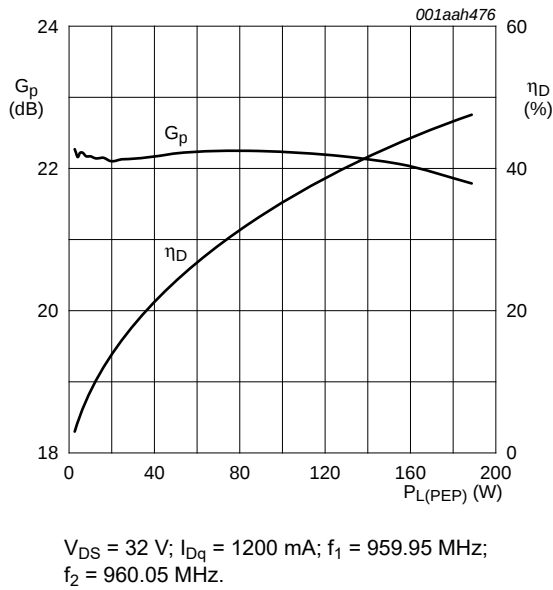
Fig 4. Power gain and drain efficiency as function of peak envelope power load power; typical values
