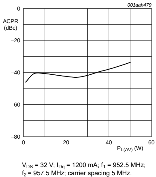
Fig 7. Adjacent power channel ratio as a function of average output power; typical values
