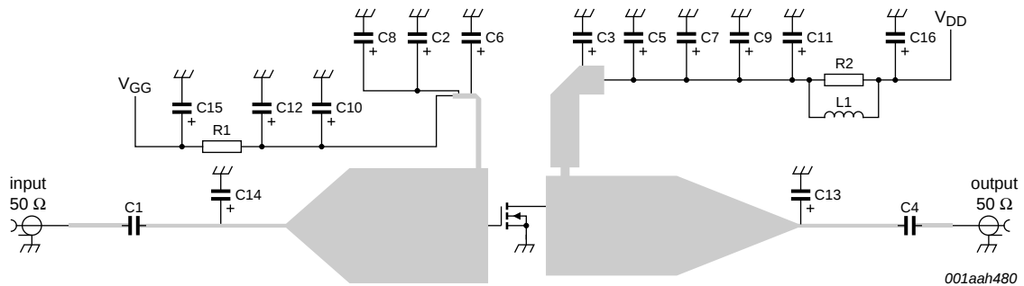
Fig 1. Test circuit for operation at 900 MHz
