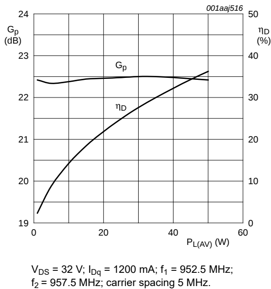
Fig 6. Power gain and drain efficiency as function of average output power; typical values
