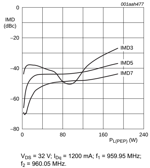
Fig 5. Intermodulation distortion as a function of peak envelope power load power; typical values
