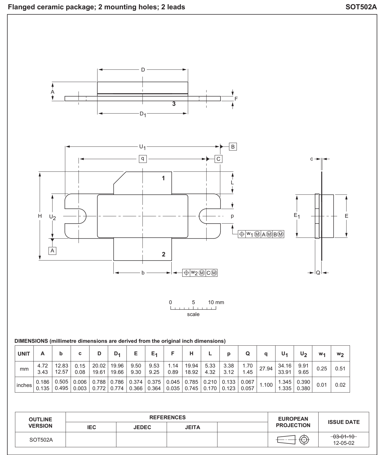
Fig 8. Package outline SOT502A
