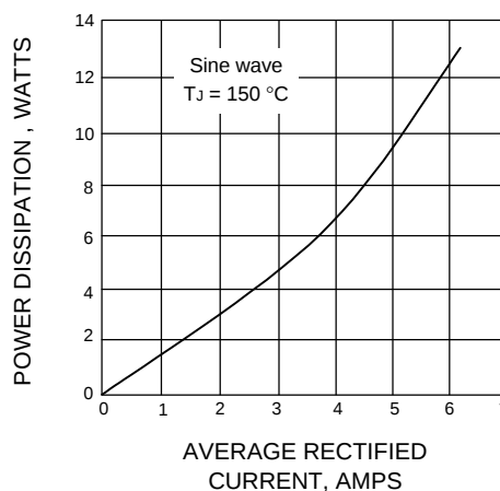
FIG.4 - POWER DISSIPATION
