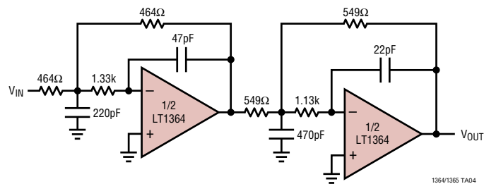
2MHz, 4th Order Butterworth Filter
