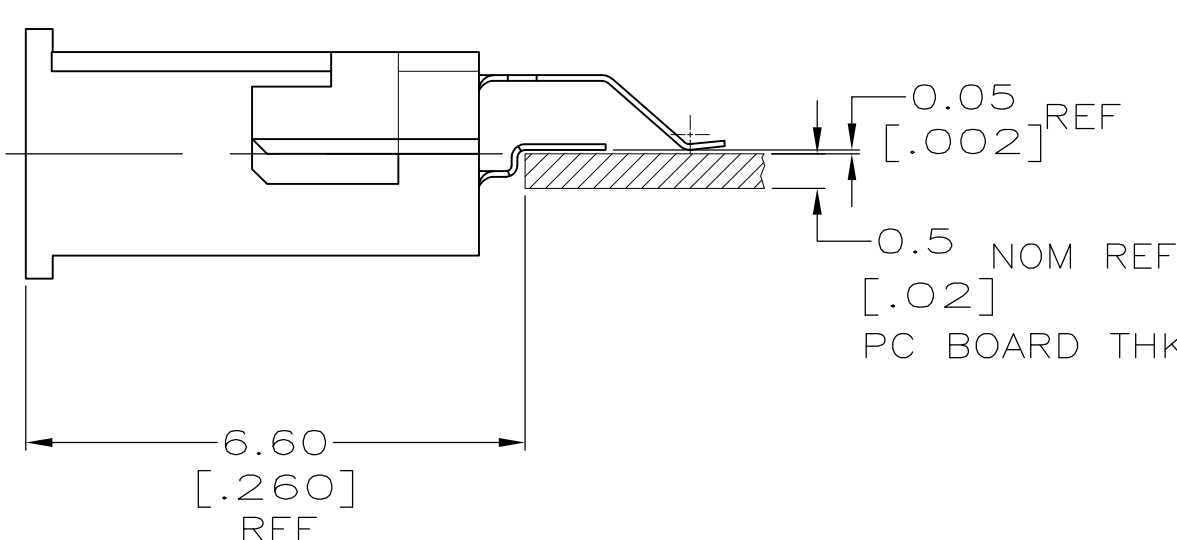
PC BOARD LOCATION SCALE 10:1
