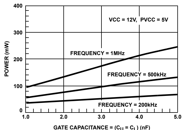
FIGURE 6. VARIABLE LOADING PROFILE (HIP6603B)
