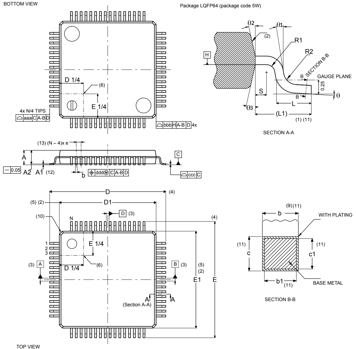
Figure 82. LQFP64 - Outline (15.)
