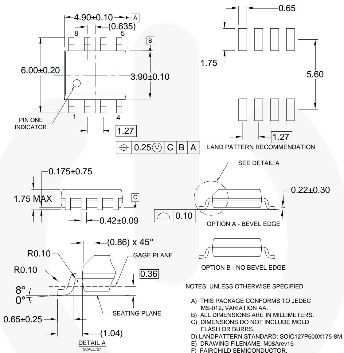
Figure 58. 8-Lead Small Outline Integrated Circuit (SOIC)
