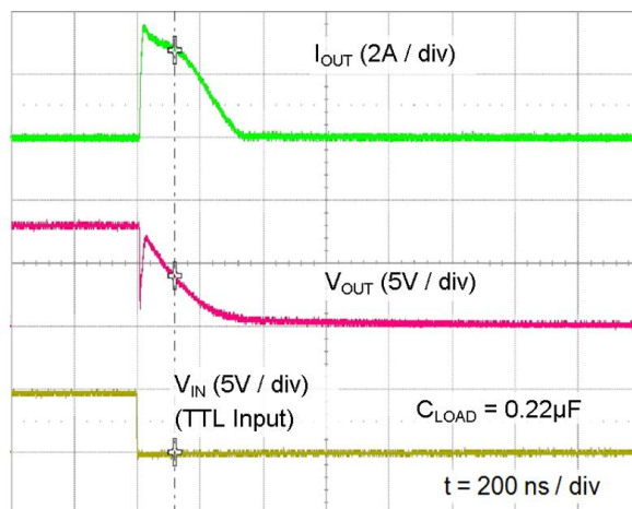
Figure 43. Quasi-Static Sink Current with V_{DD}=12\text{ V}^{(16)}
