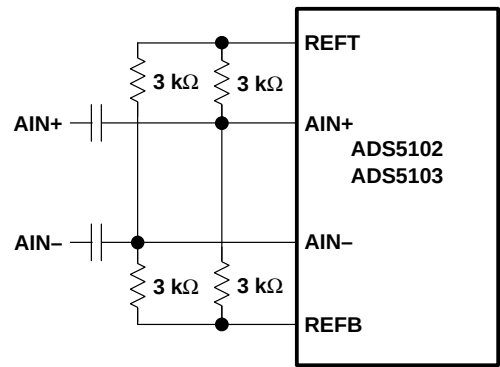
Figure 33. Driving the Analog Inputs
