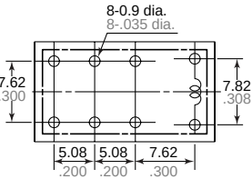
Tolerance: ±0.1 ± .004 Schematic (Bottom view)
