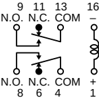
Tolerance: ±0.1 ± .004 Schematic (Bottom view)
