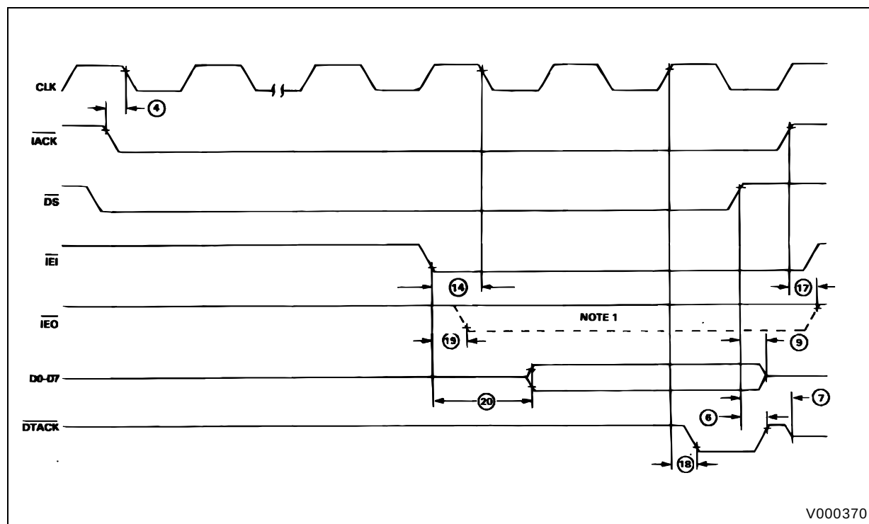
Figure 24 : Interrupt Acknowledge Cycle ( \overline{\text{IEI}} high).
