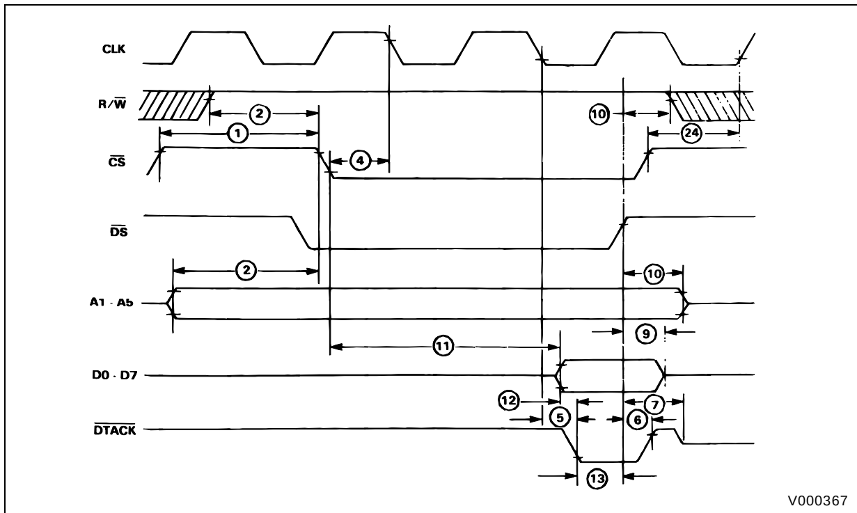
Figure 22 : Write Cycle.
