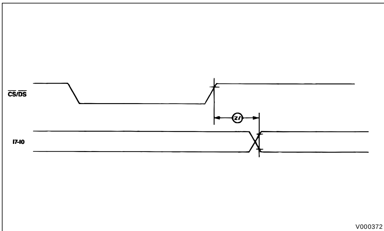
Figure 26 : Port Timing.
