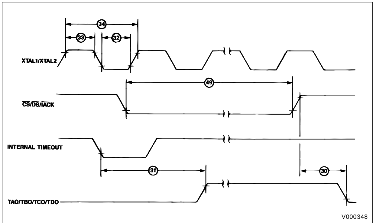
Figure 30 : Reset Timing.
