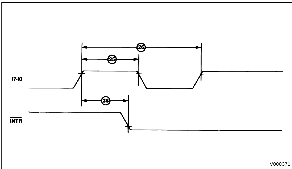
Figure 25 : Interrupt Timing.
