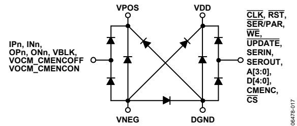
Figure 19. ESD Protection Map
