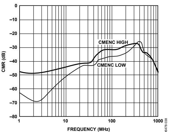
Figure 31. Common-Mode Rejection
