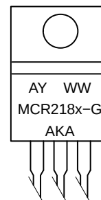
TO-220AB CASE 221A-09 STYLE 3
