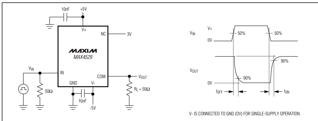
Figure 2. Switching Time
