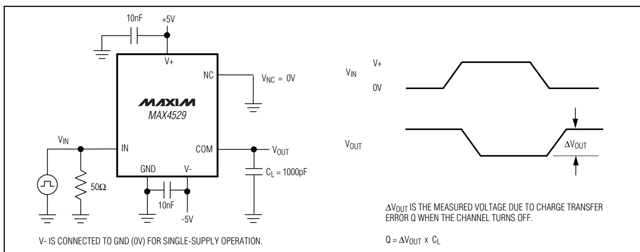
Figure 3. Charge Injection
