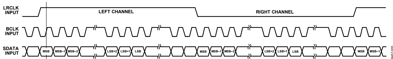
Figure 5. Left-Justified Mode
