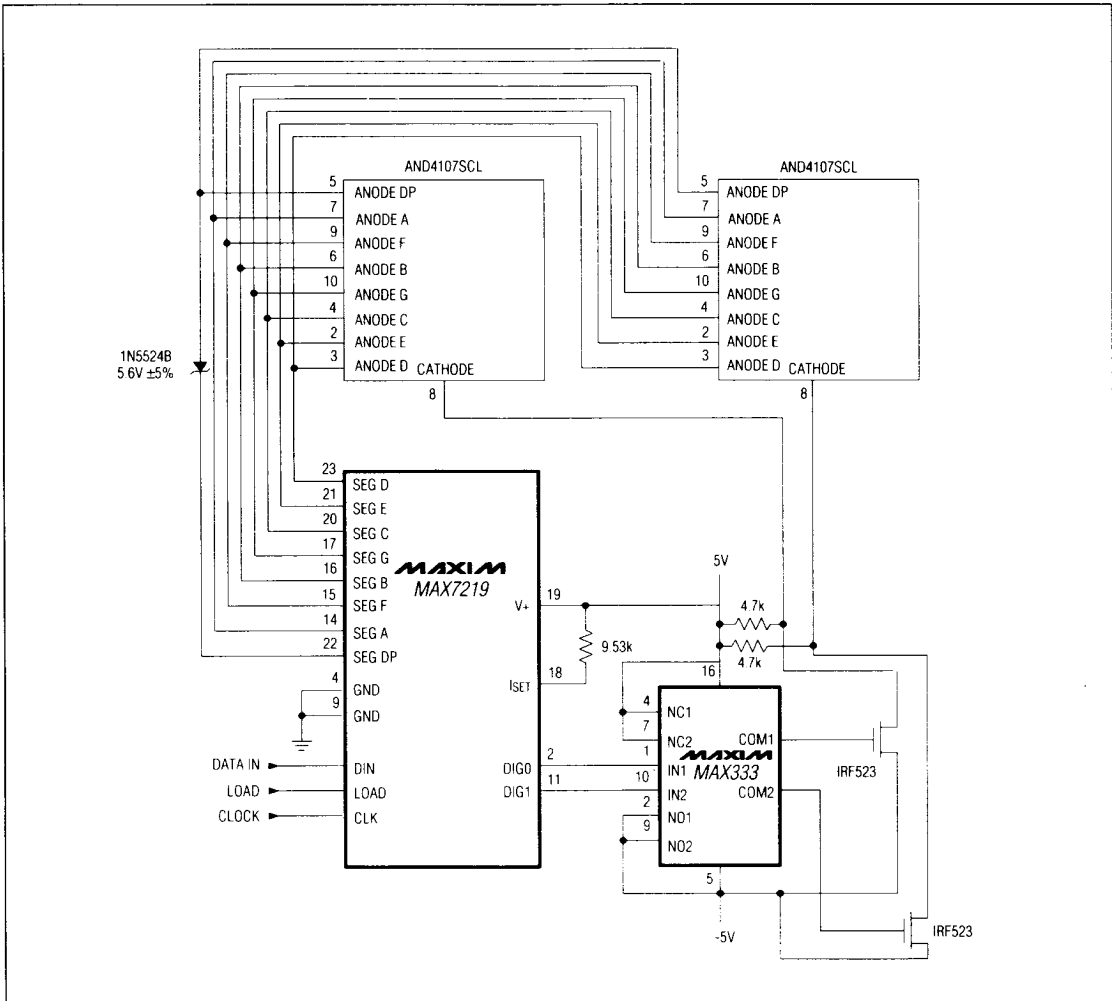
Figure 2. MAX7219 Driving 4 Inch Displays
