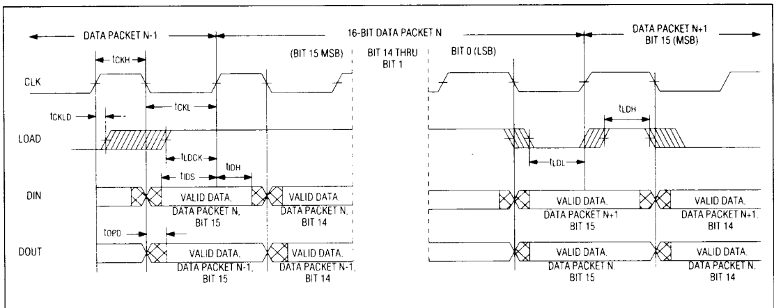
Figure 1. Timing Diagram
