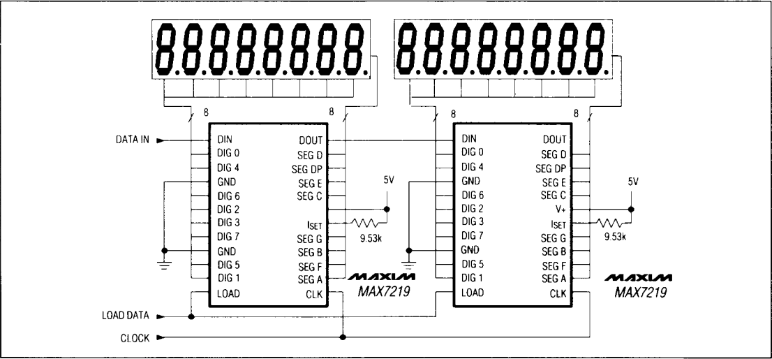
Figure 3. Cascading MAX7219s to drive 16 7-segment LED digits.
