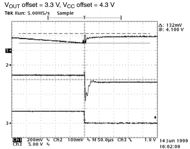
Figure 9. V CC Power-down (V AUX = 3.3 V)
