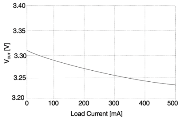
Figure 2. Load Regulation
