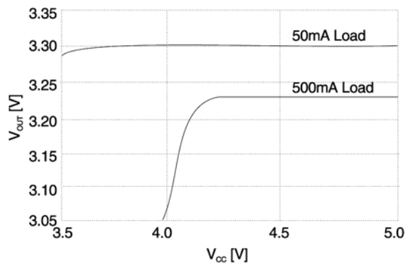
Figure 1. Dropout Characteristics
