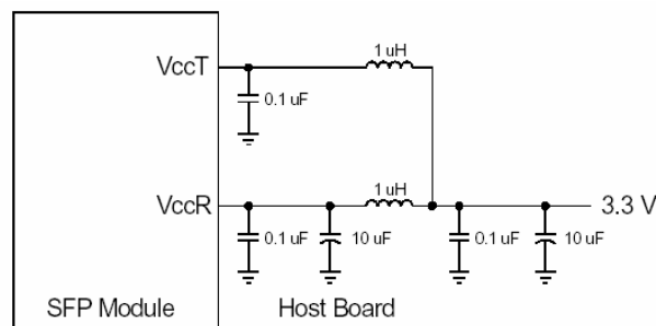
Figure 2, Recommended Host Board Power Supply Circuit
