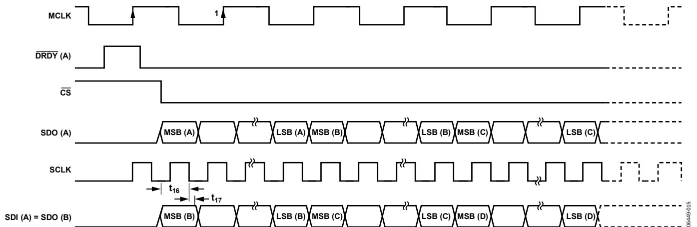
Figure 38. Daisy-Chain SDI Setup and Hold Timing
