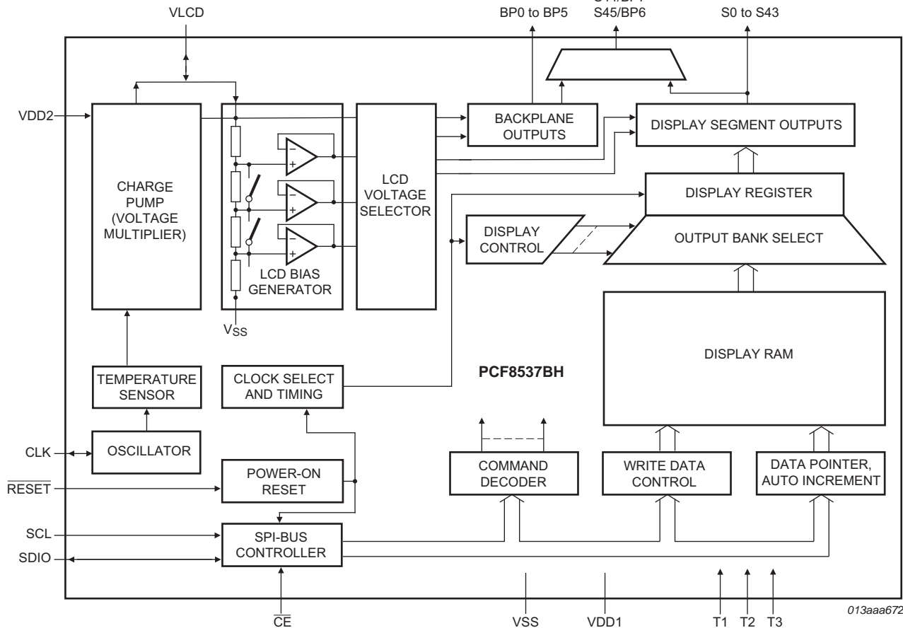
Fig 2. Block diagram of PCF8537BH
