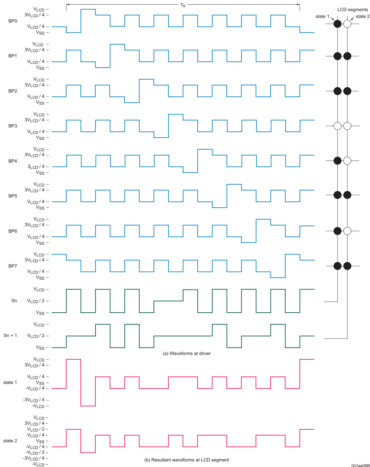
Fig 30. Waveforms for 1:8 multiplex drive mode with \frac{1}{4} bias (line inversion mode)
