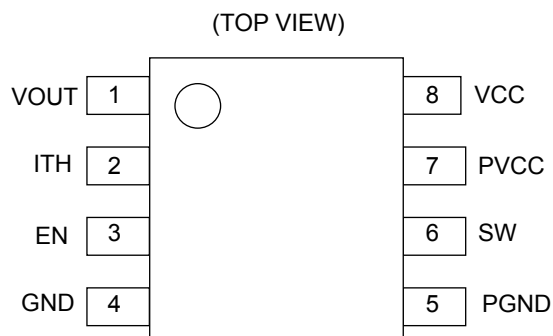
Figure 2. Pin Configuration
