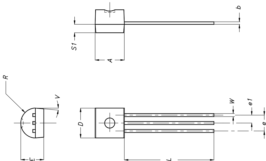
Figure 10. TO-92 package outline
