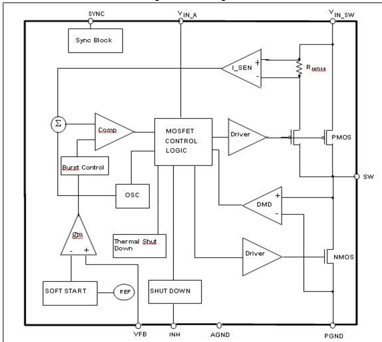
Figure 8. Block diagram
