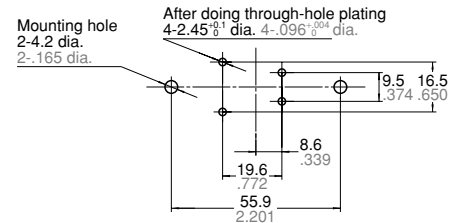
Mounting dimensions
