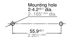
Mounting dimensions
