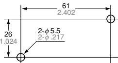
Mounting dimension
