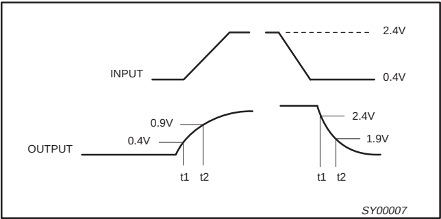
Waveform 4. Slew Rate Waveforms Voltage Waveforms (Input pulse rise and fall time are 3ns, 150ns < pulse width < 10 \mu s, for both a Low to High and a High to Low transition.) Slew Rate measured between 0.4V and 0.9V - rising. Slew Rate measured between 2.4V and 1.9V - falling. Slew Rate measured at TP1.
