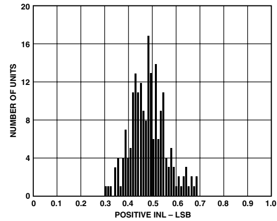
TPC 3. Typical Positive INL Distribution (199 Units)
