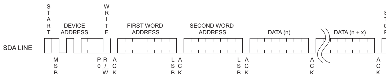
Figure 9-2. Page Write
