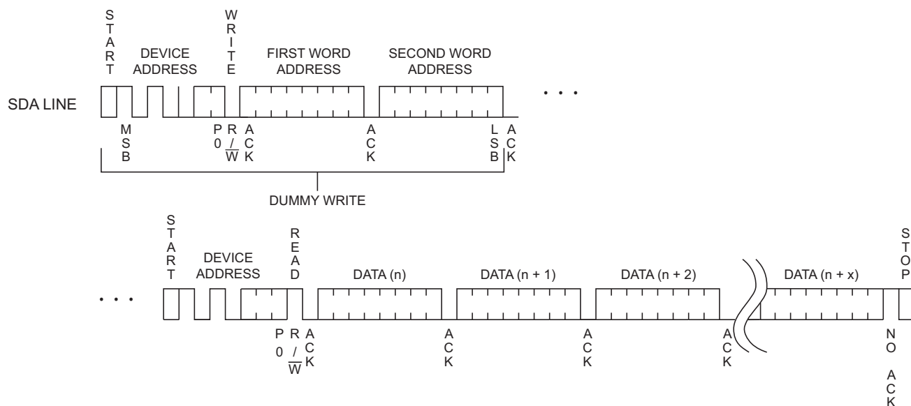
Figure 9-5. Sequential Read
