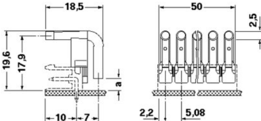
Dimensioned drawing
