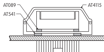
Splash Cover
