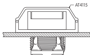
Snap-in Mount
