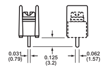
14 Printed Circuit
