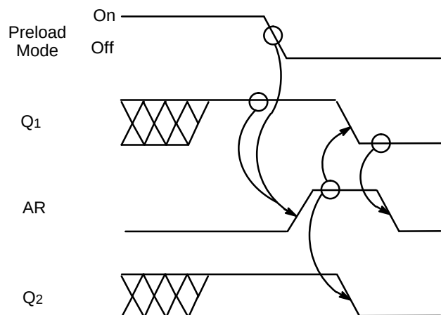
Figure 8. Preload/Reset Conflict
