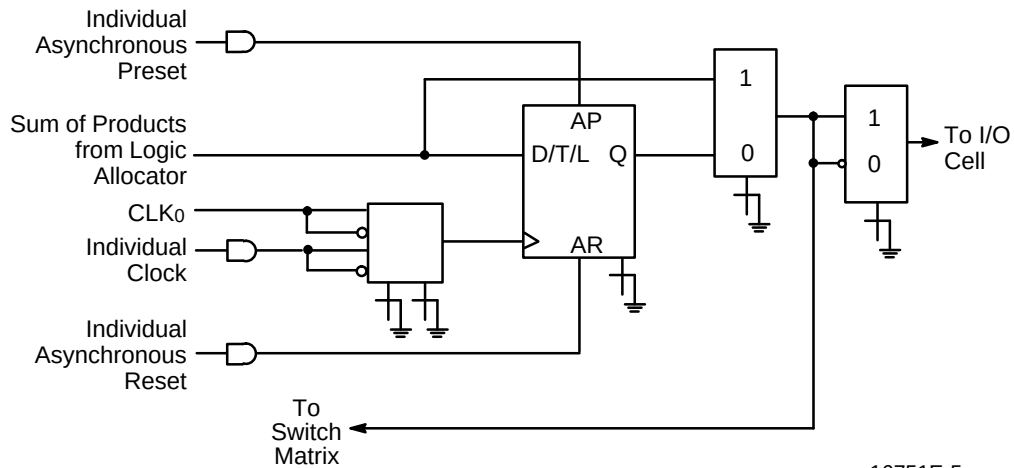
Figure 3. Output Macrocell
