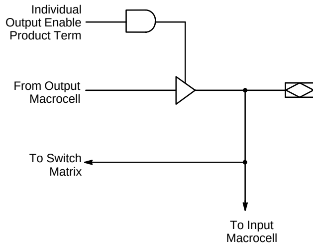
Figure 7. I/O Cell
