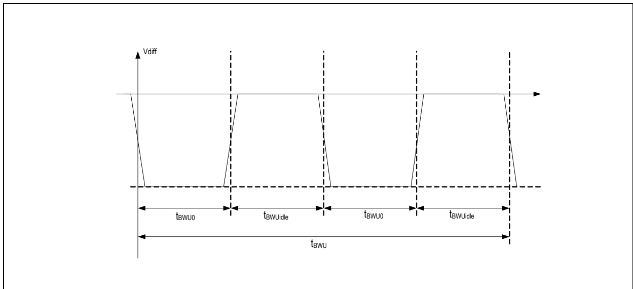
Figure 8. Signal for Wake-up Pattern Recognition
